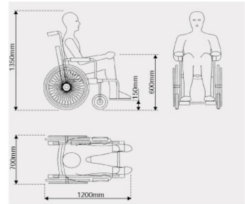
Diagram Wheelchair dimension - reference wheelchair
